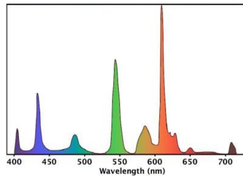
Figure 4: Light sources produce varying amounts of light in different wavelengths. Labs often measure and describe these traits by using Spectral Power Distribution (SPD) graphs.
