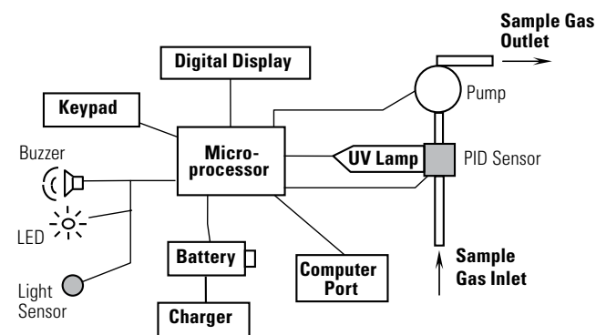
FIGURE 2.5.1. Overall PID instrument schematic
