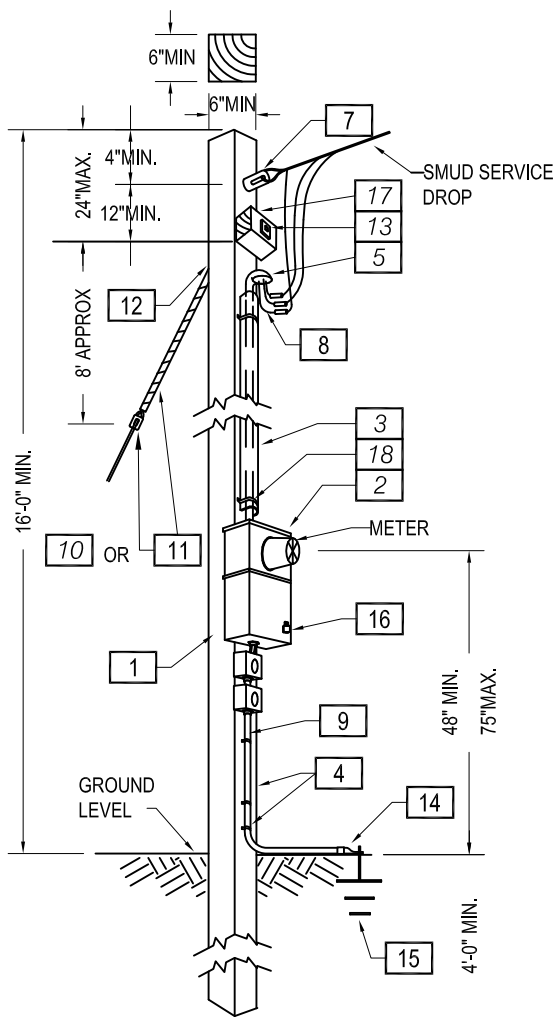
SERVICE DROP CABLE TO RECEPTACLES
