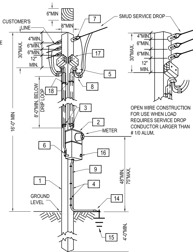
SERVICE DROP CABLE TO OVERHEAD LINE
